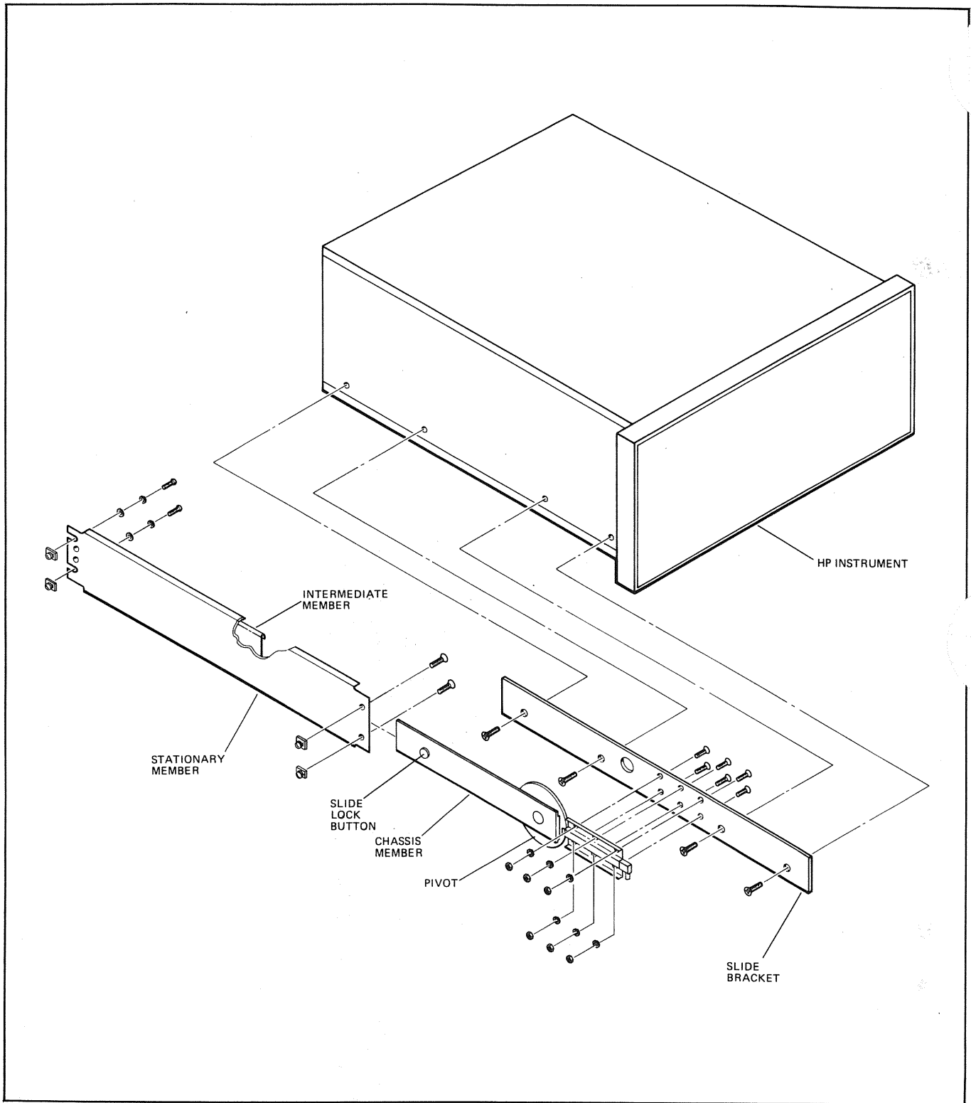
Figure 1. Installation Details
