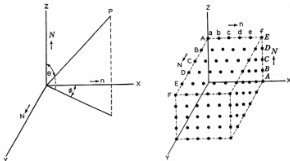
Fig. 21—General case of linear antenna arrays.
