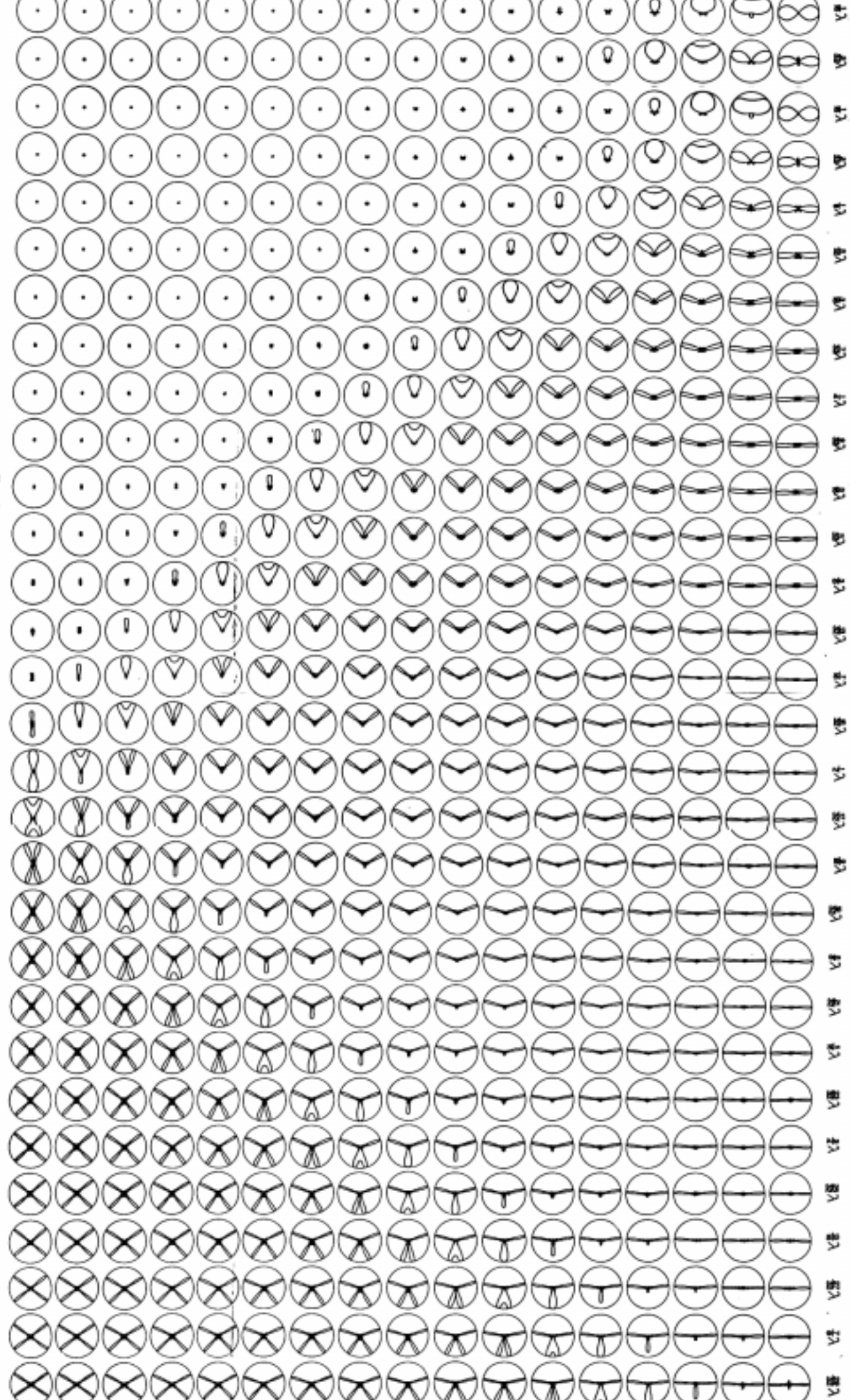
Fig. 4—Directional morphologic changes in an array of neurons stimulated. Separation in wave-lengths \lambda along the top. Phase difference in periods T at the left.
