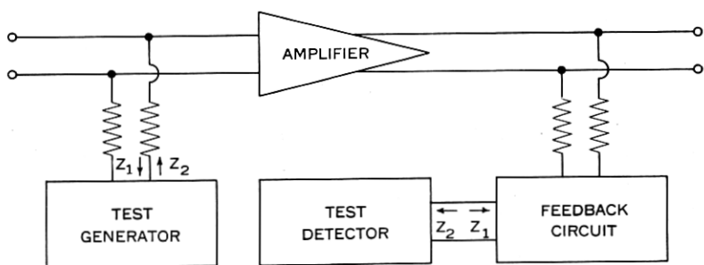
Fig. 5—Test for stability of feedback amplifier.
