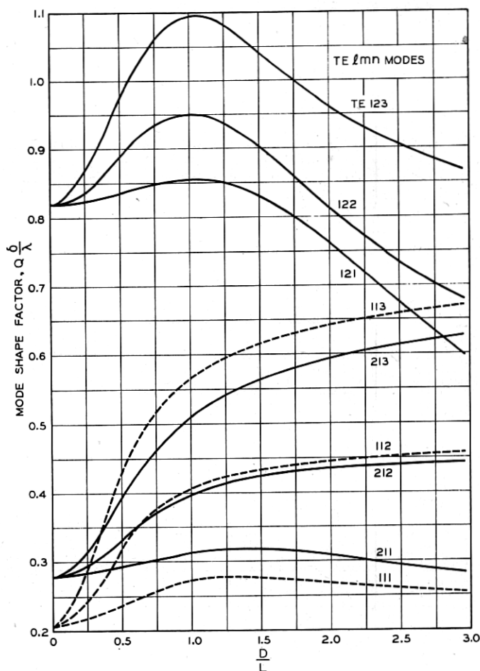
Fig. 4—Mode-shape factors \left(Q/\lambda\right) as a function of diameter to length ratio \left(D/L\right) for circular cylinder resonator — TE modes with l > 0 .
