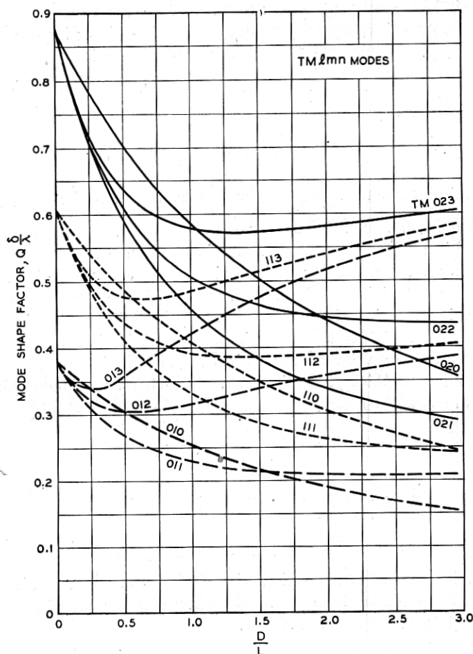
Fig. 2—Mode-shape factors \left(Q_{\delta}/\lambda\right) as a function of diameter to length ratio \left(D/L\right) for circular cylinder resonator— TM modes.
