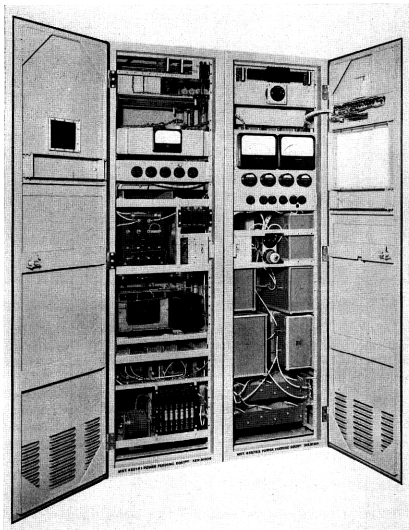
Fig. 7 — Power equipment.
