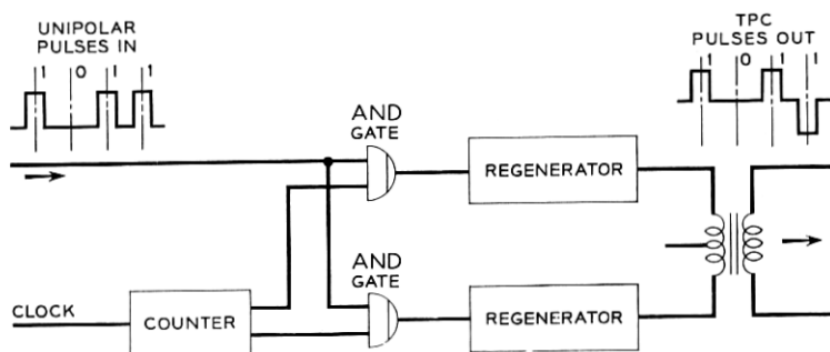
Fig. 10 — TPC converter.
