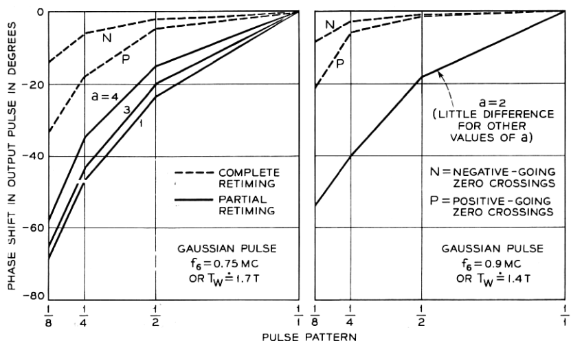
Fig. 5 — Pattern effects — Gaussian pulse: (a) f_6 = 0.75 \text{ mc} , (b) f_6 = 0.90 \text{ mc} .
