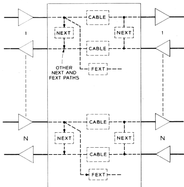
Fig. 6 — "Channel" for N PCM systems.
