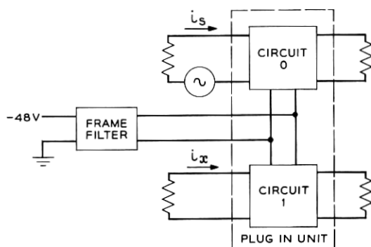
Fig. 14 — Attenuation of crosstalk signal i_x in ckt. 1 over input signal i_s in ckt. 0 when coupling is via common frame filter and power wiring as well as adjacency of components on mounting unit.
