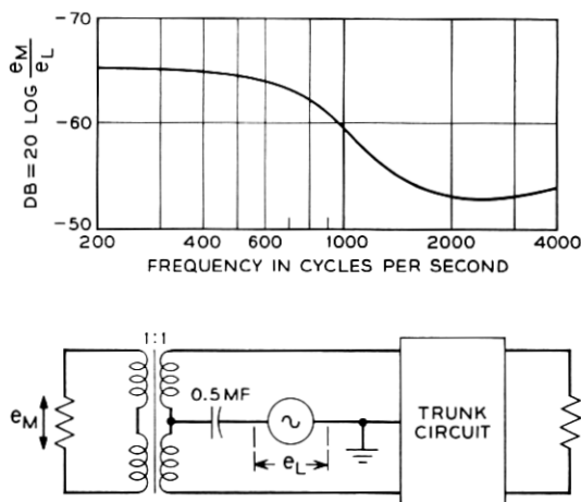
Fig. 13 — Longitudinal balance of trunk transmission circuit. Balance in \text{db} = 20 \log [e_{\text{metallic}}/e_{\text{longitudinal}}] when measured as shown.
