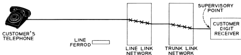
Fig. 2 — A line supervised at customer digit receiver during dialing.
