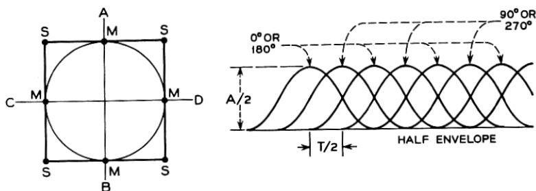
Fig. 8 — Duobinary FM.
