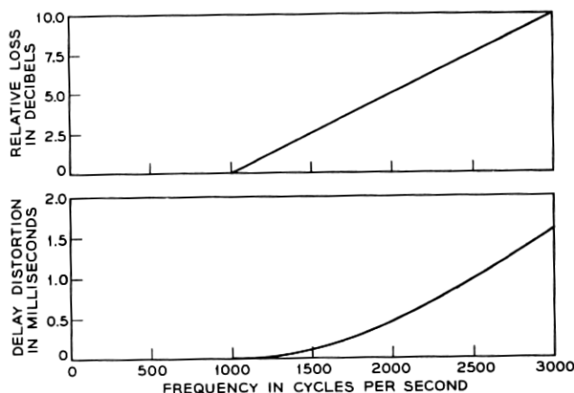
Fig. 12 — Amplitude and delay distortion characteristics used to distort the signal patterns shown in Fig. 11.
