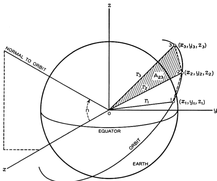
Fig. 4 — The orbit and Gaussian triangles.
