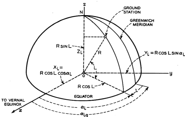
Fig. 5 — Ground station coordinates.
