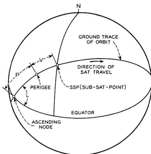
Fig. 1 — Geometry for determining the subsatellite point.
