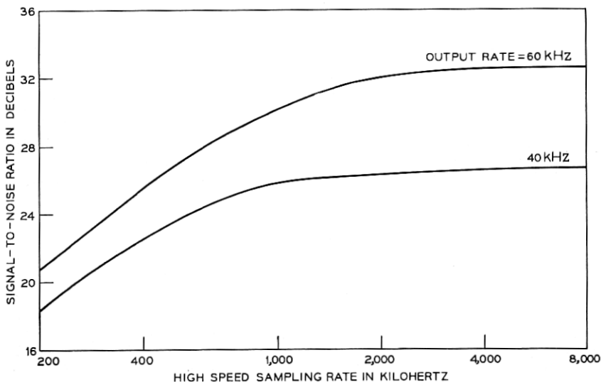
Fig. 2—Performance characteristics.
