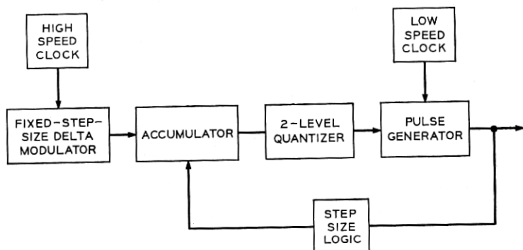
Fig. 3—Simplified implementation.
