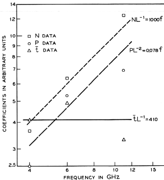
Fig. 7—Coefficients of P , N , and l characteristics versus frequency.
