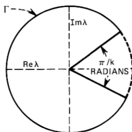
Fig. 2—Proof of lemma.
