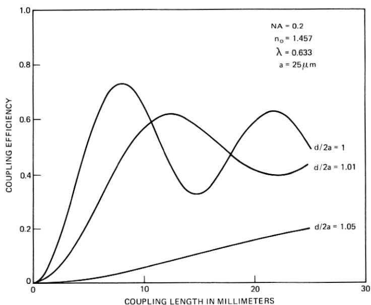
Fig. 4—Coupling efficiency vs coupling length.
