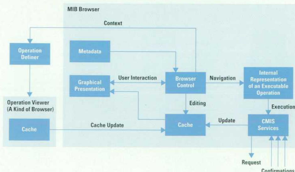
Fig. 3. The design of the MIB browser.
