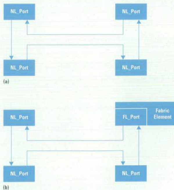
Fig. 2. Fibre Channel arbitrated loop topology. (a) Private Loop. (b) Public loop.
