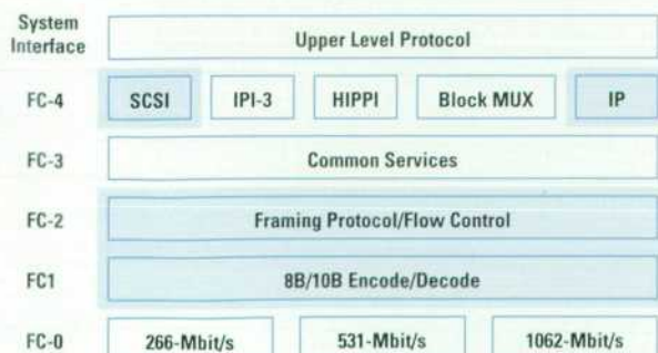
Fig. 7. Fibre Channel's five layers.
