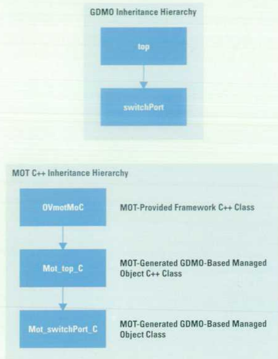
Fig. 8. The C++ GDMO inheritance hierarchies of the GDMO-defined switchPort managed object class.
